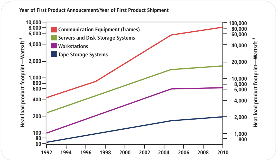
The Uptime Institute Measurement of Heat Load
