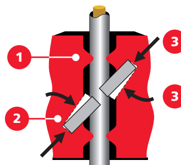
ADC KRONE's LSA Plus Technology
