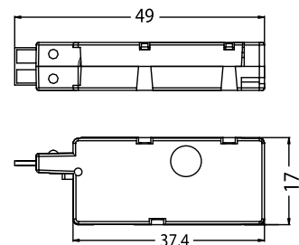
Component Dimensions
